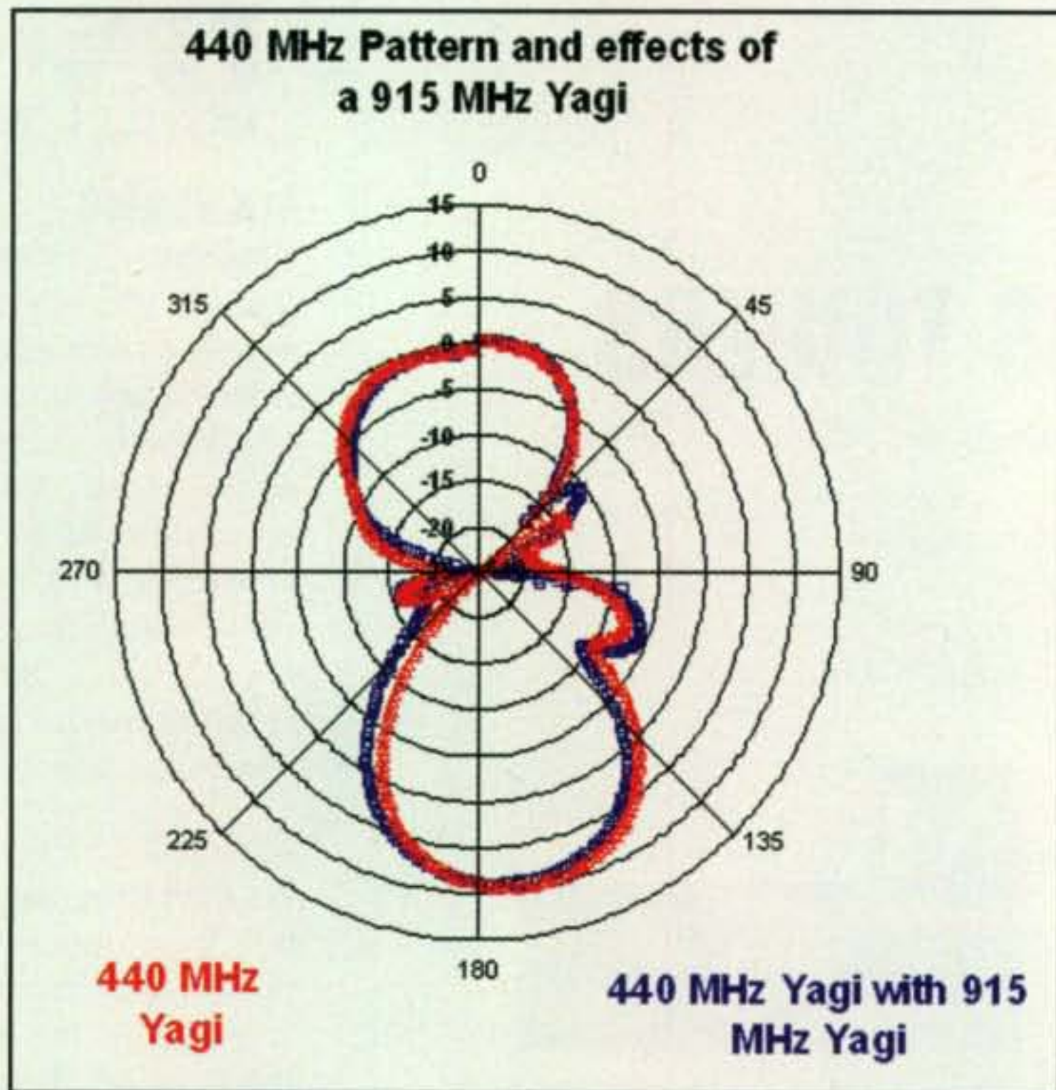
Plot 1— 440-MHz Yagi with and without a close-spaced 915-MHz Yagi (see text for details).
