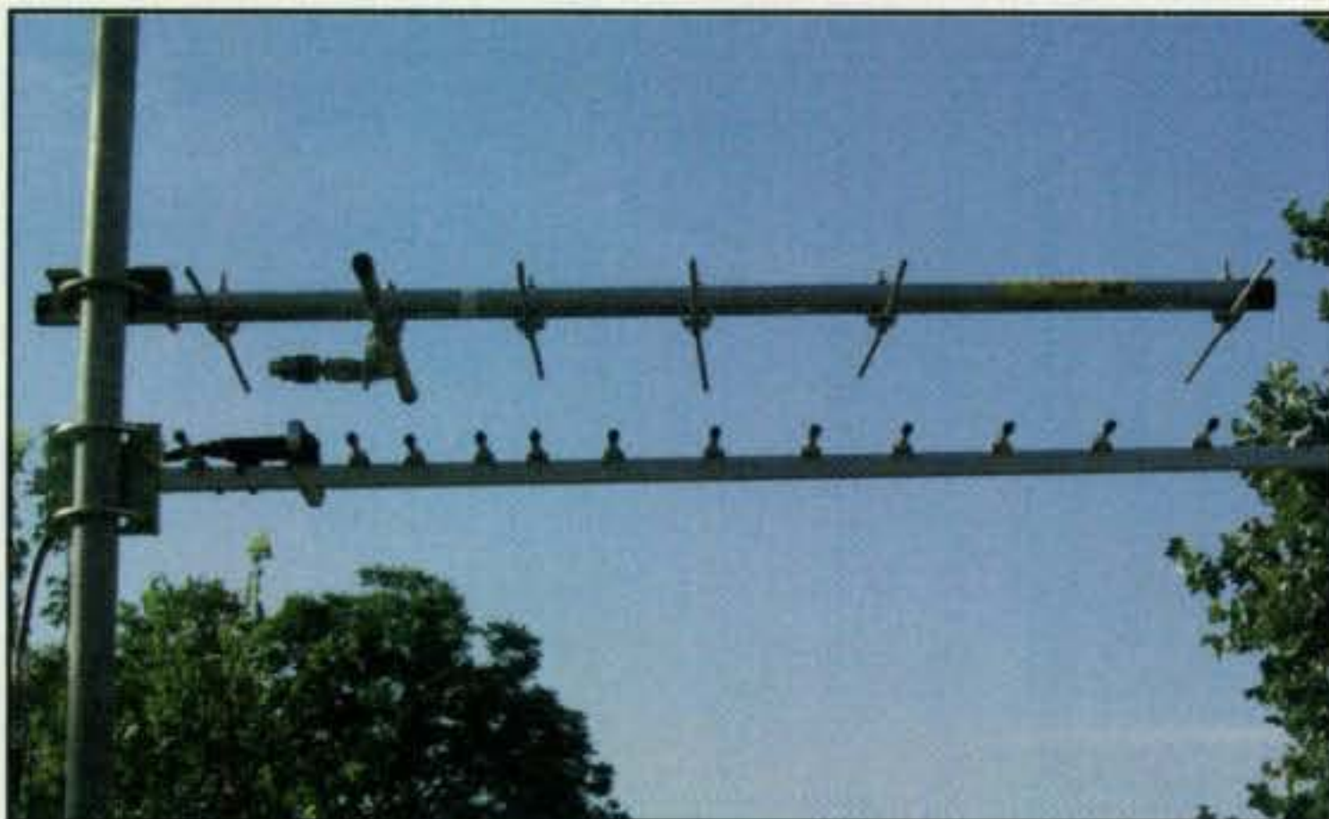
Photo D— Measuring a 915-MHz Yagi and its interaction with a 440-MHz Yagi.
